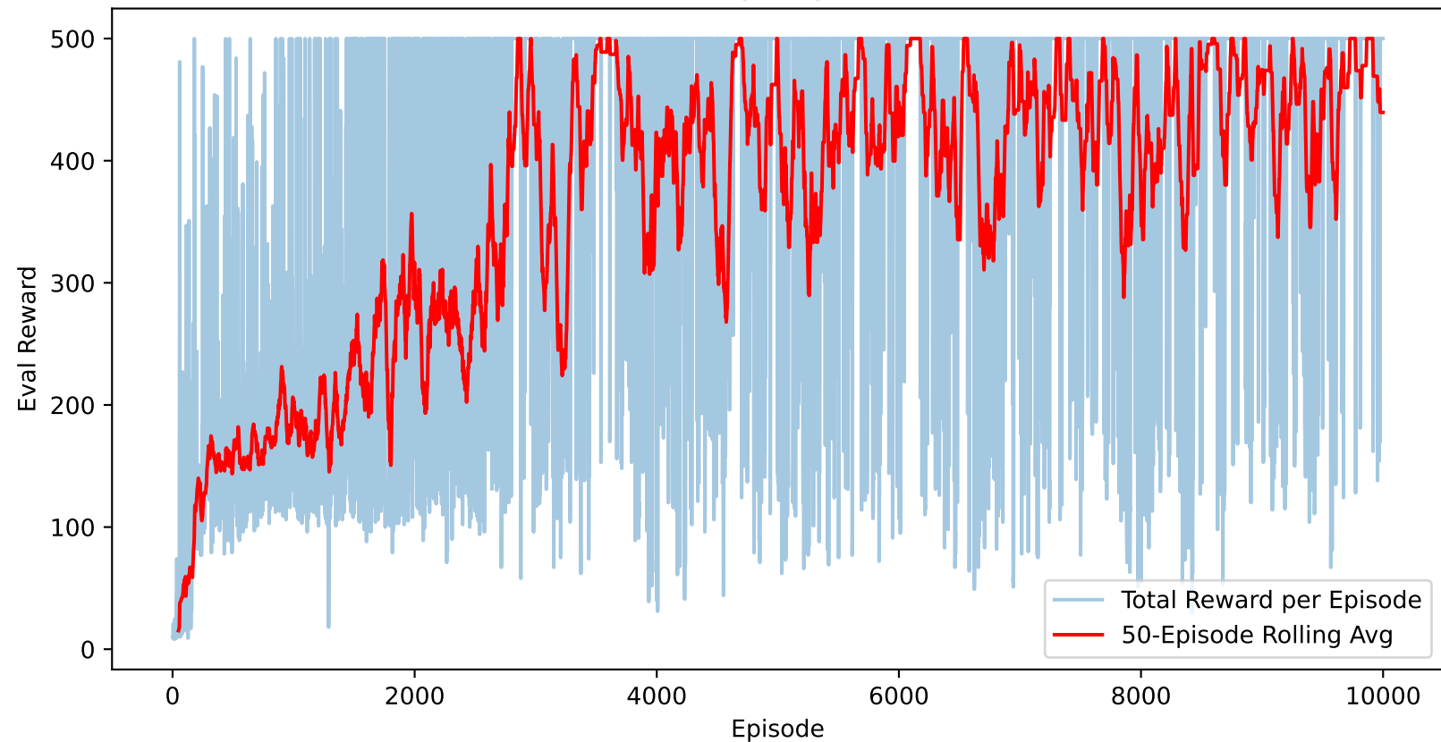
CartPole PPO Training Progress (Eval Rewards)
