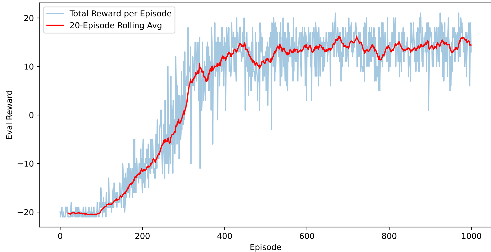
Pong DDQN Training Progress (Eval Rewards)
