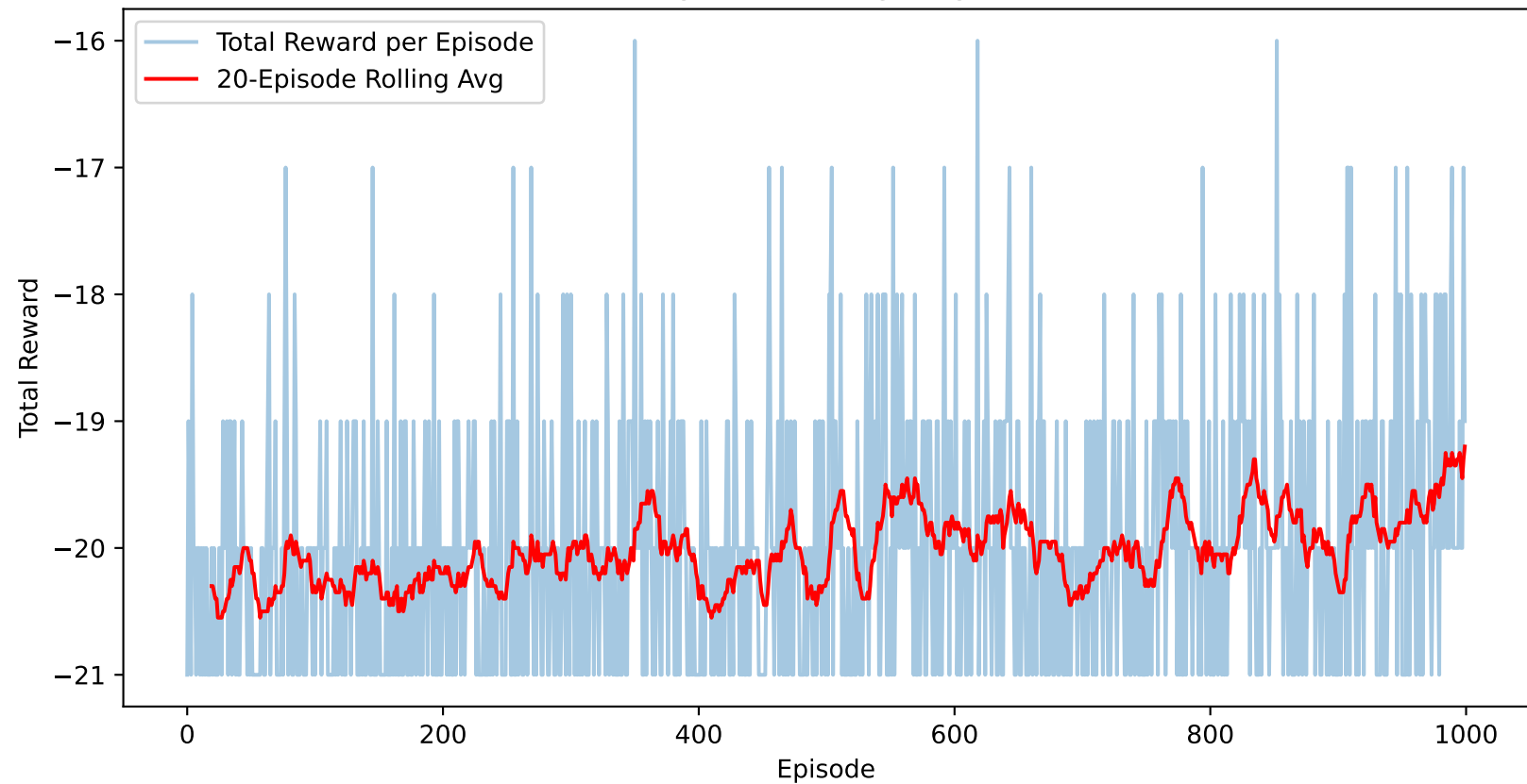
Pong PPO Training Progress
