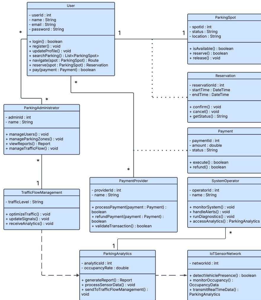
Parking System UML Class Diagram
