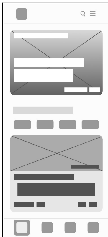
Home Page
