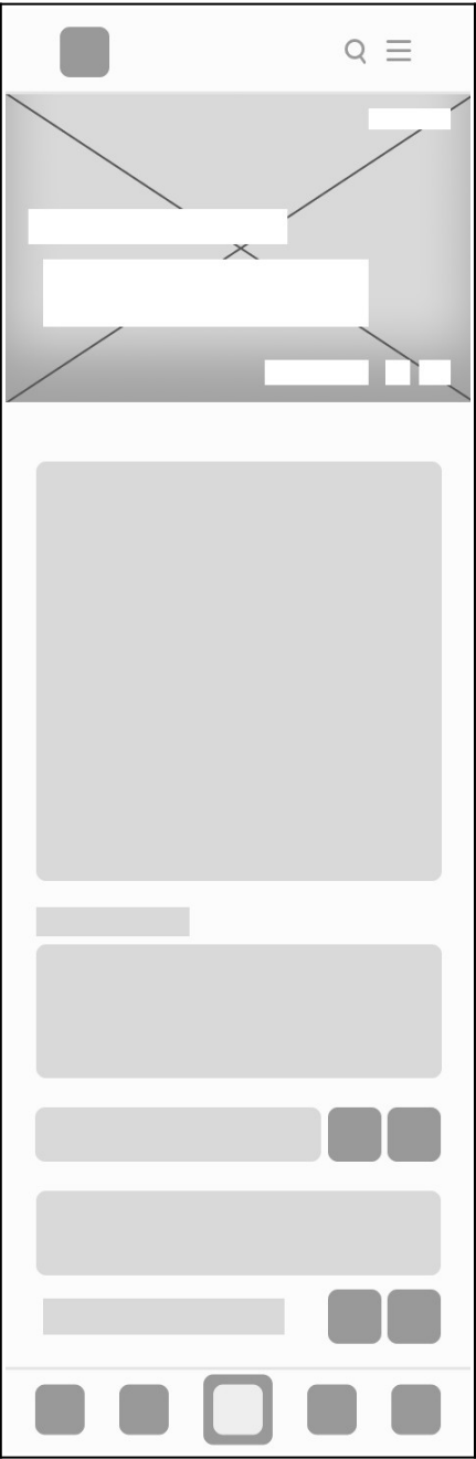
Post viewer
