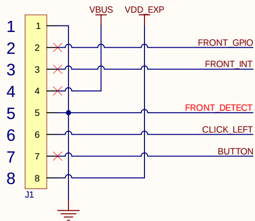
LEFT CONNECTOR
