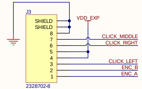
CONNECTOR
