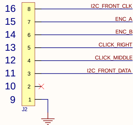
RIGHT CONNECTOR
