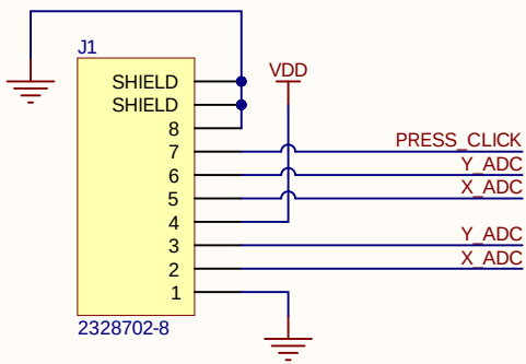
CONNECTOR
