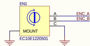
ENCODER (SCROLL WHEEL)
