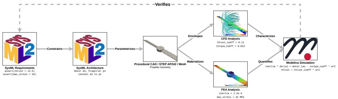
Figure 1. The Code-Centric Digital Thread: reconciling SysML v2 architecture, procedural CAD geometry, and Modelica physical dynamics with closed-loop requirements verification.
