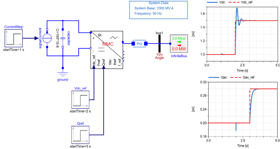
Figure 1. DCvoltageModeTest: the DCvoltageModeMMCStation between a DC-side current source and an AC grid equivalent (left); DC voltage tracking of the V_{dc,ref} step (top right) and reactive power tracking of the Q_{ac,ref} step (bottom right).
