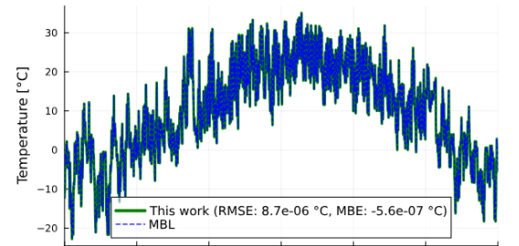
Outdoor dry-bulb temperature (SimpleHouse0)
