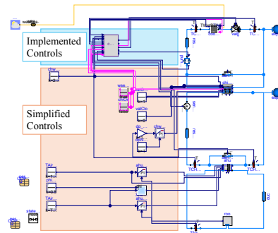
Figure 1. A full system model with around half of the implemented control blocks replaced with simple control signals.
