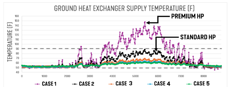
Figure 2 Conceptual results comparing the GHX Leaving Temperatures between a traditional sizing tool (Case 1) and a more accurate Modelica-based simulation (Cases 2-5).
