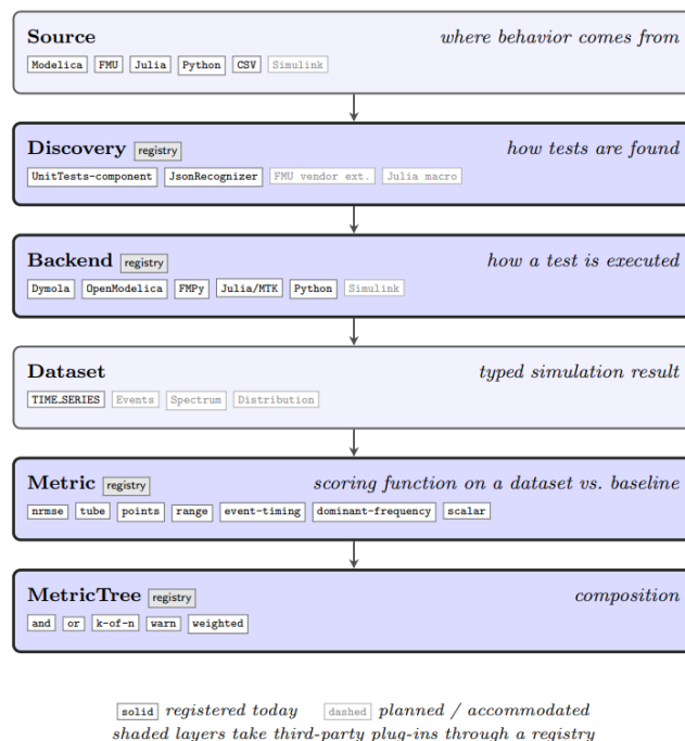
Figure 1. The six-layer plug-in architecture of DSTF. Every layer has a defined interface, and new recognizers, simulators, metrics, or combinators install into the registry of their layer without disturbing the others.
