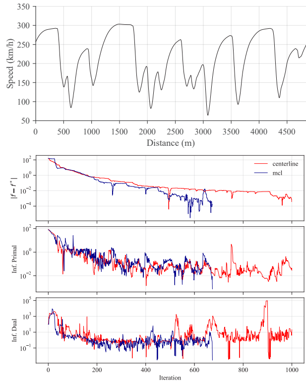
Figure 2. Singapore optimization results: optimized speed trace (top) and IPOPT iteration histories for centre-line and minimum-curvature references (bottom).
