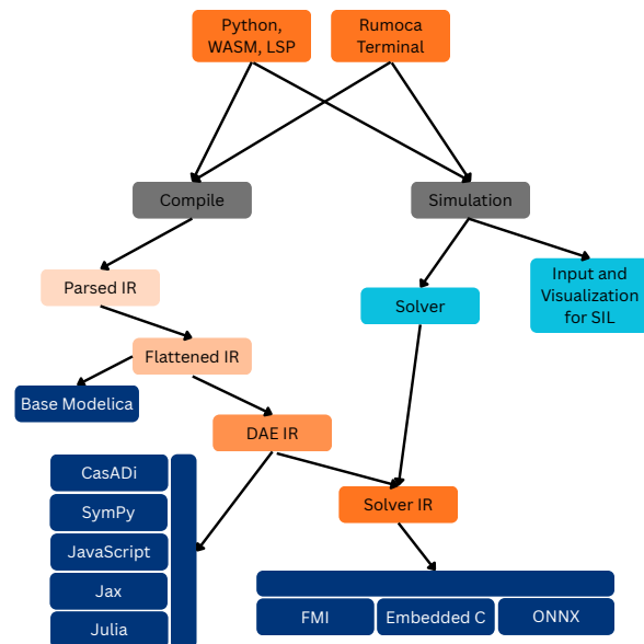
Figure 1. Rumoca’s architecture. Compile and Simulation are peer activities, each callable from the CLI, language server, Python, or WebAssembly frontends; the IRs feed the code generators and the native Rust runtime.
