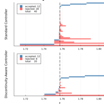
Figure 2. Trial steps near a discontinuity. Discontinuity awareness reduces rejected steps from 28 to 8.
