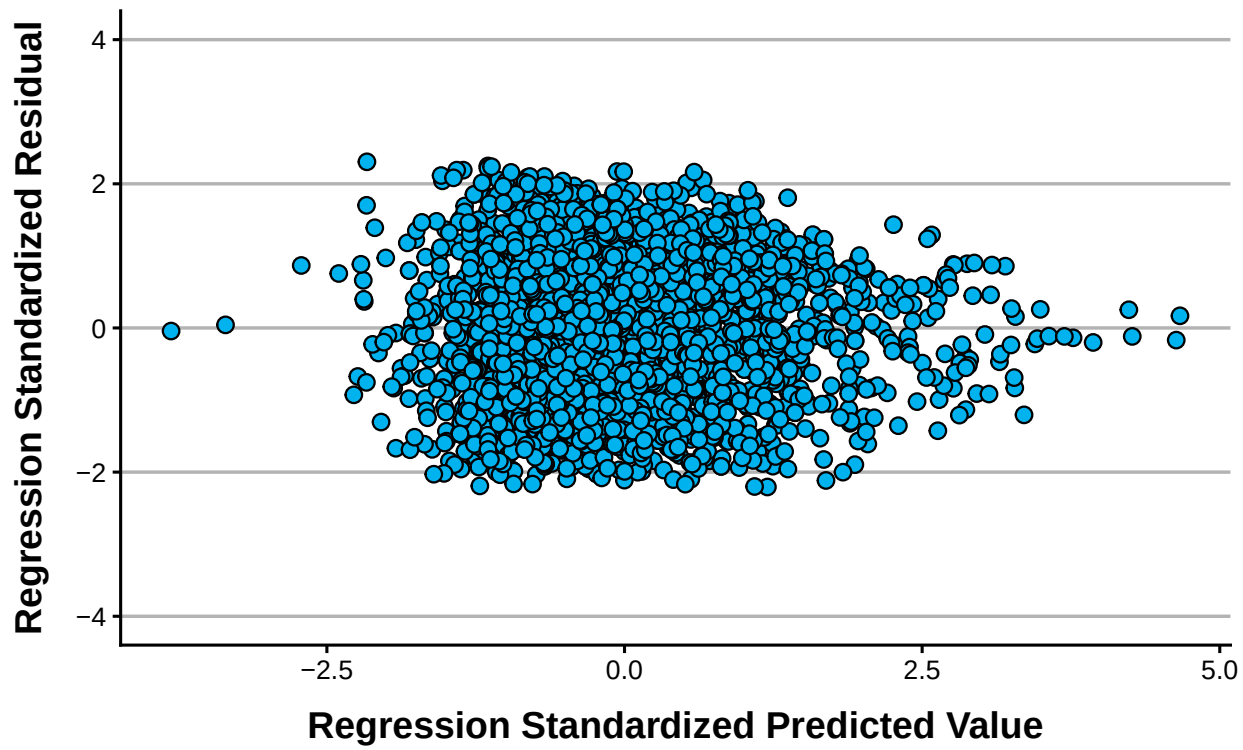
Scatterplot Dependent Variable: LN_PRICE
