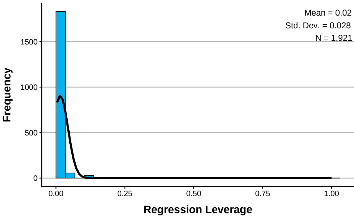
Histogram Dependent Variable: LN_PRICE
