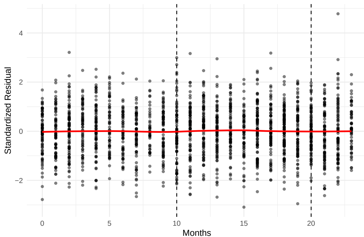
Residuals for LN_PRICE (No ECFs) Model
