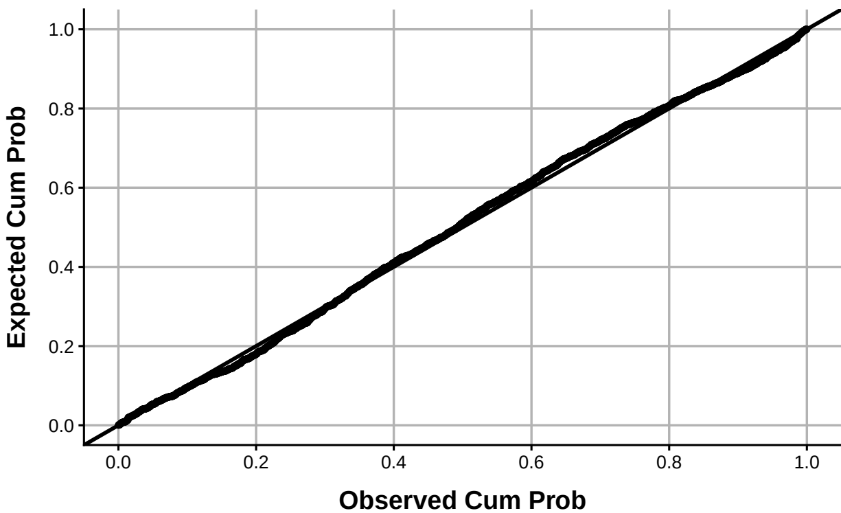
Normal P-P Plot of Regression Standardized Residual Dependent Variable: LN_PRICE
