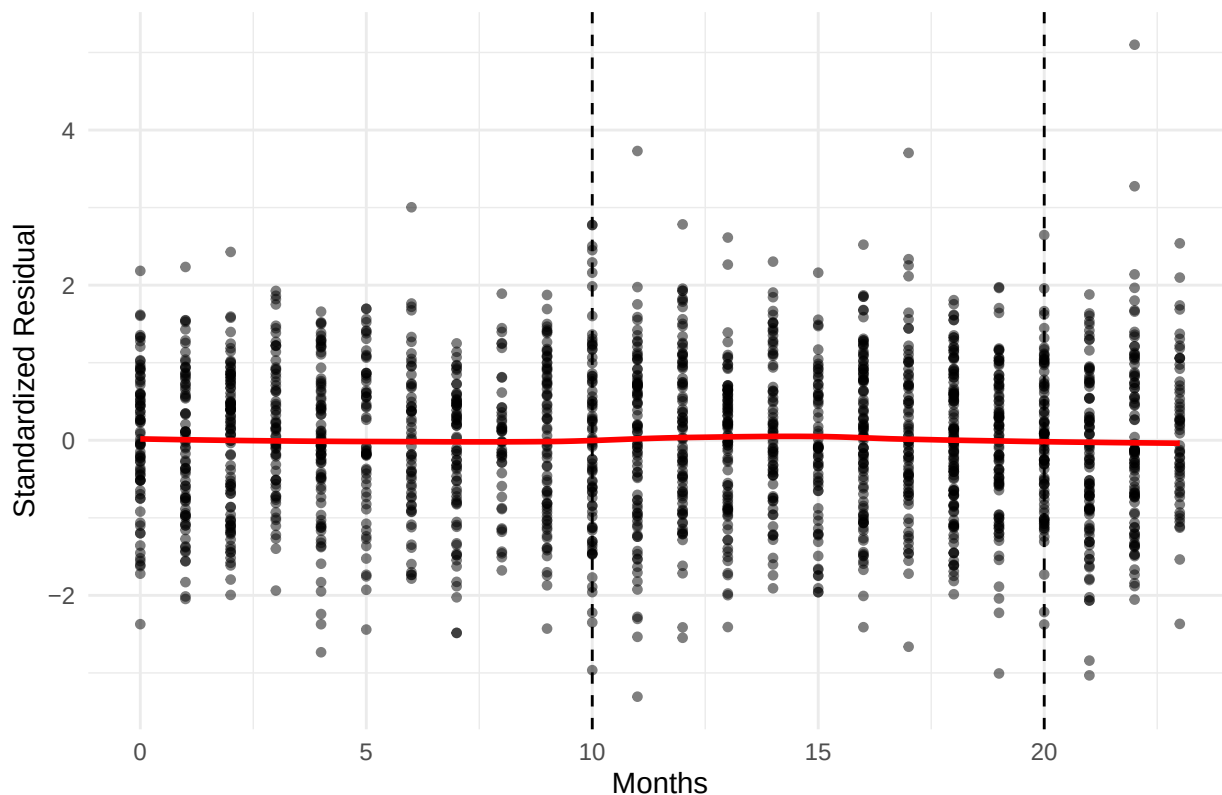
Residuals for LN_PRICE Model
