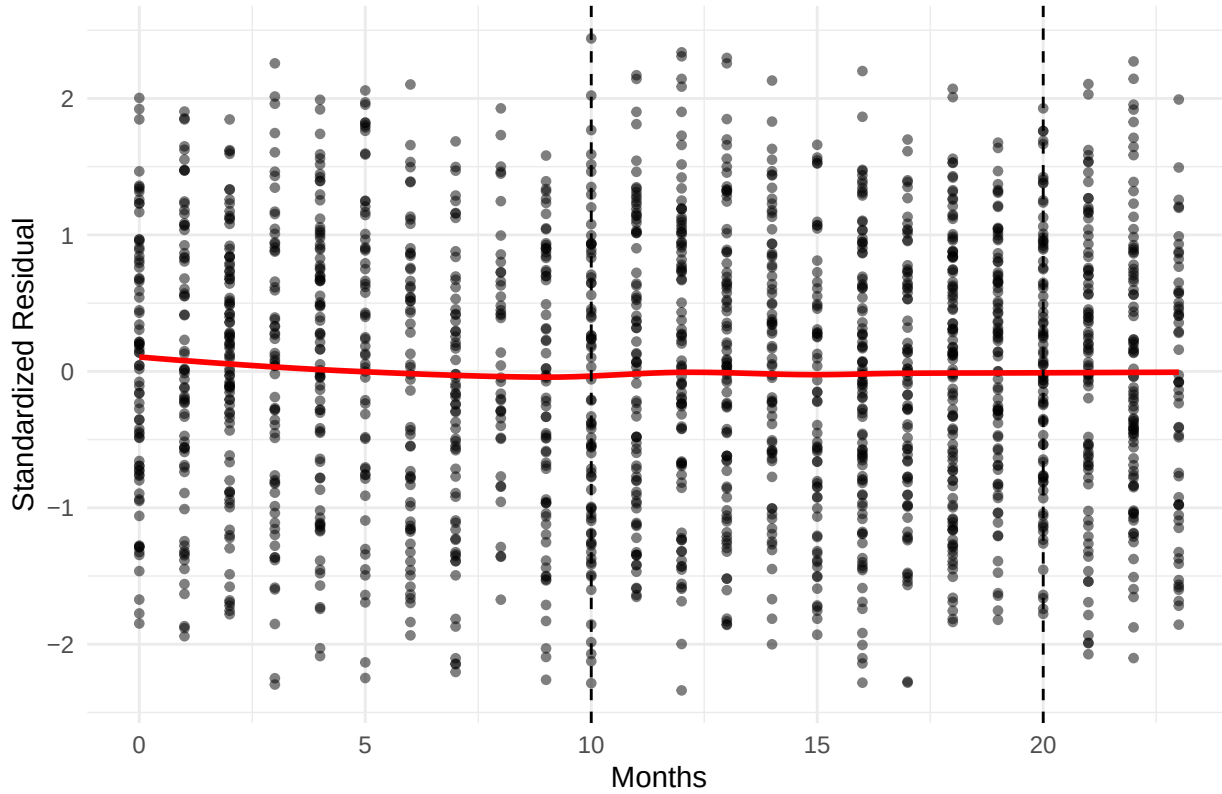
Residuals for LN_PRICE (Inliers) Model
