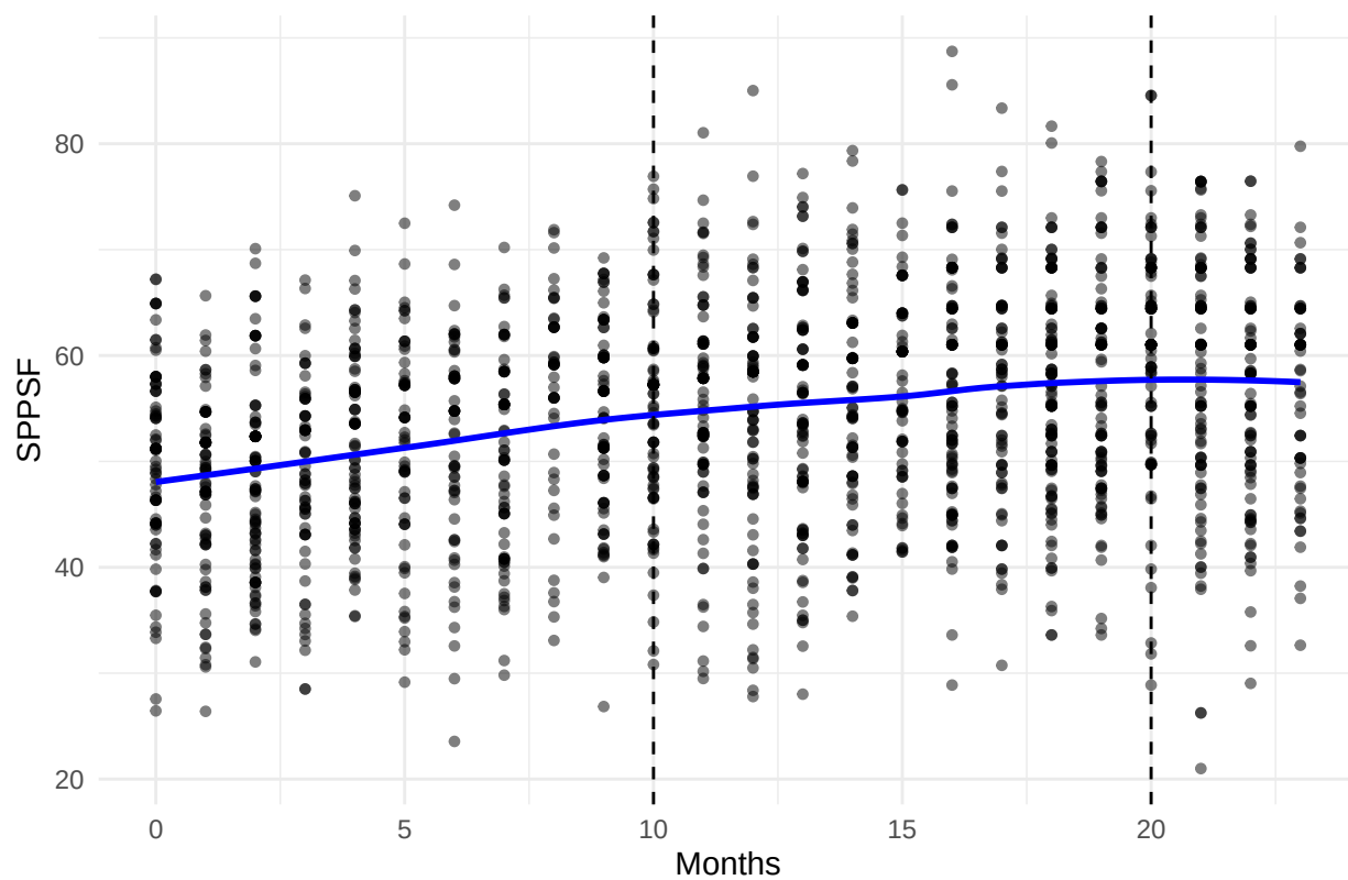
Months vs Predicted SPPSF – LN_SPPSF Model
