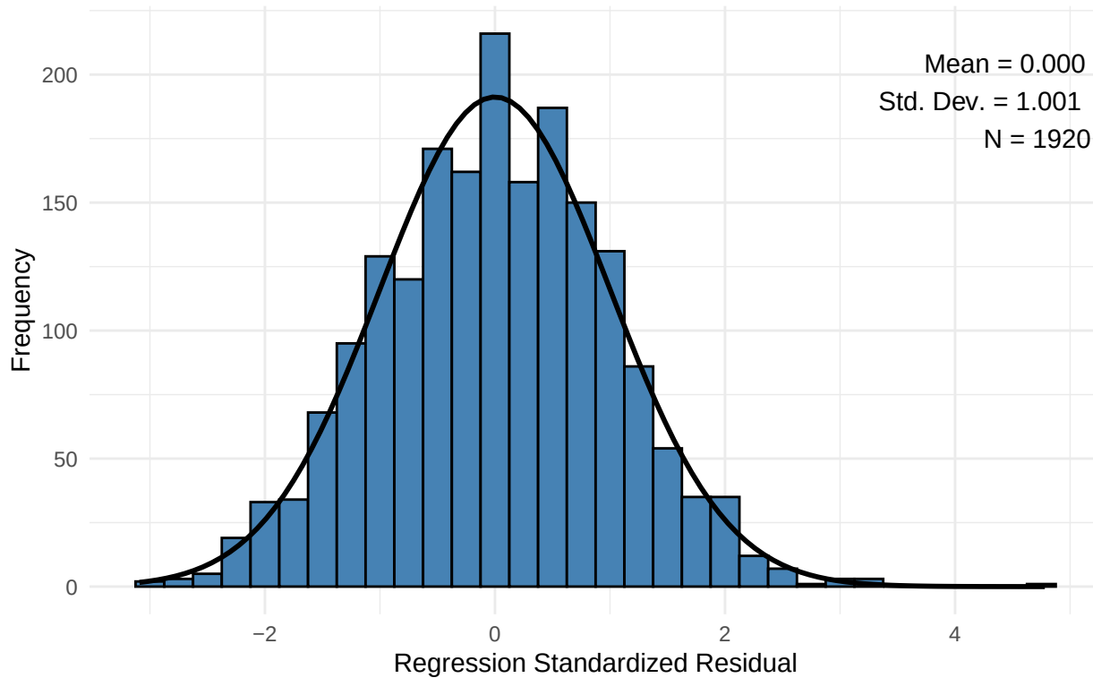
Histogram Dependent Variable: LN_PRICE (No ECFs)
