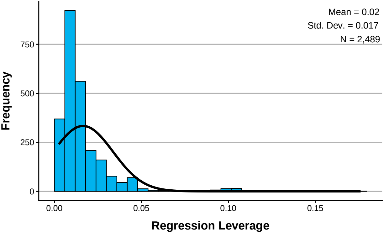
Histogram Dependent Variable: LN\ PRICE
