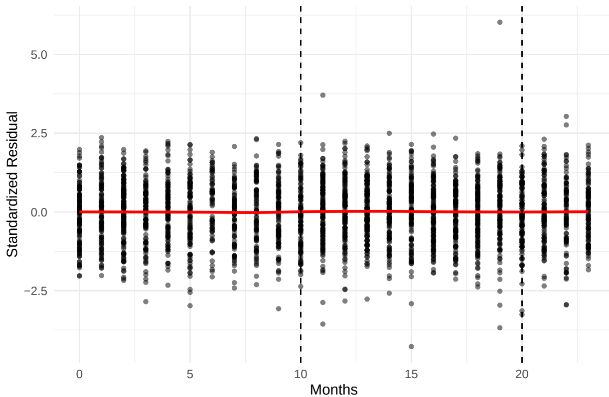
Residuals for LN_SPPSF Model
