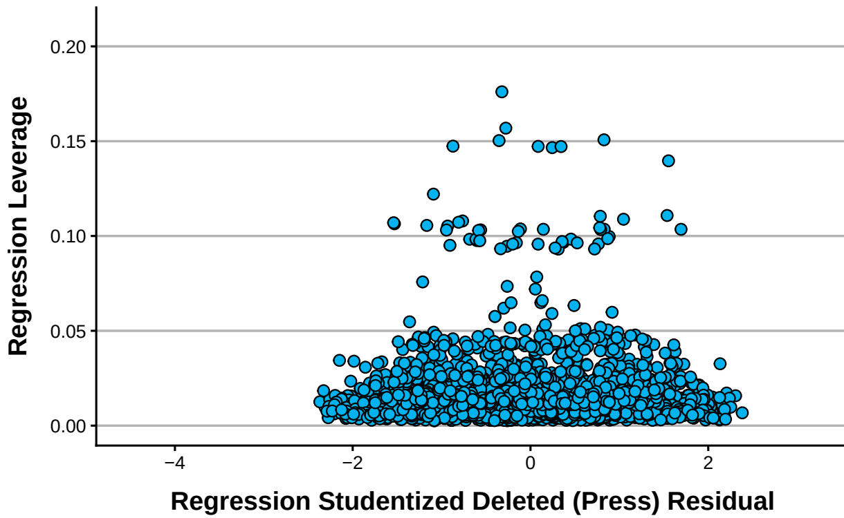
Scatterplot Dependent Variable: LN_PRICE
