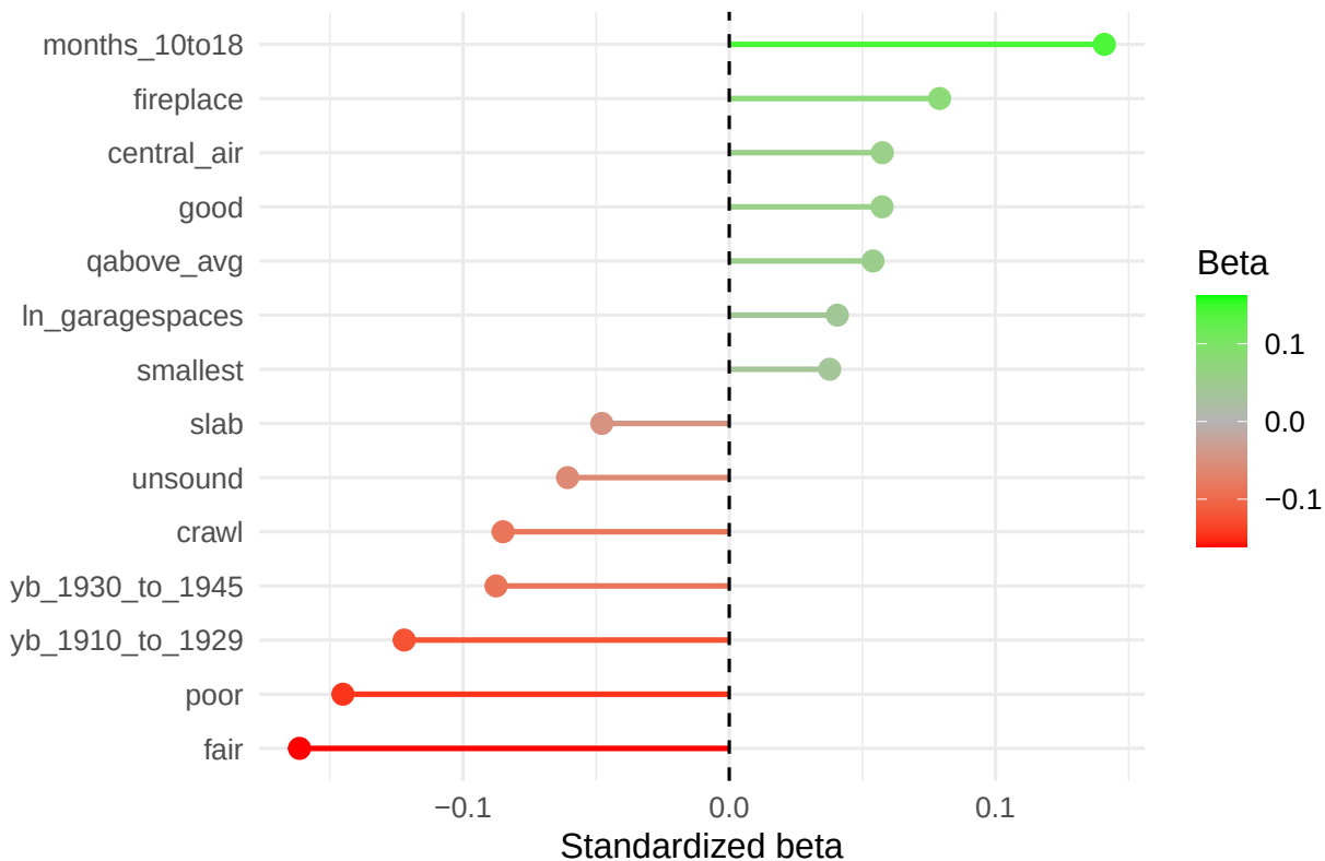
District 1 | LN_SPPSF Model Standardized Beta Values
