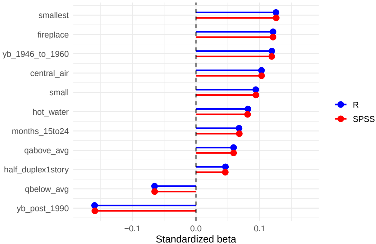
District 4 | Model I Beta Coefficient Comparison: SPSS vs R
