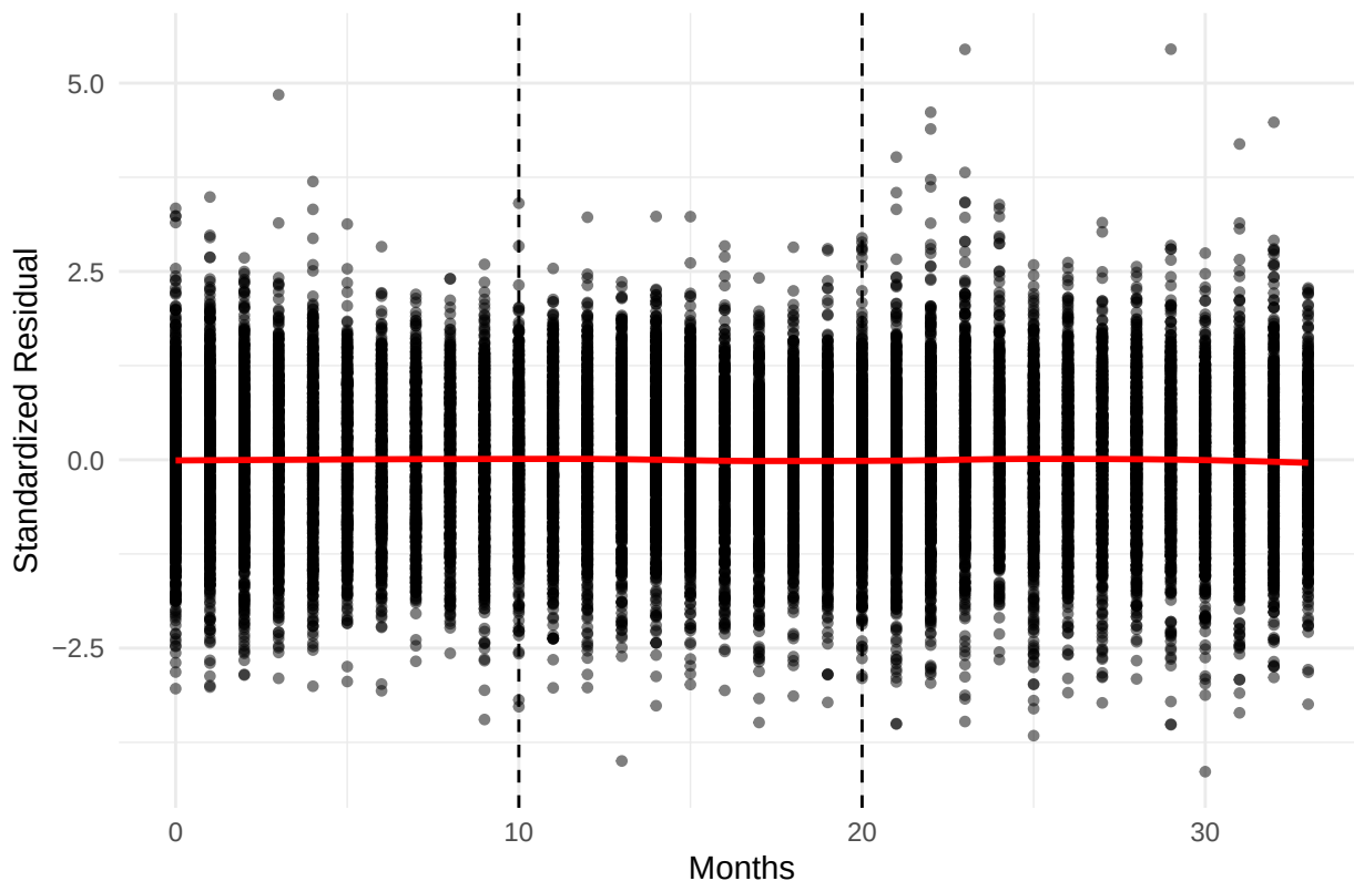
Residuals for LN_SPPSF Model + Geo
