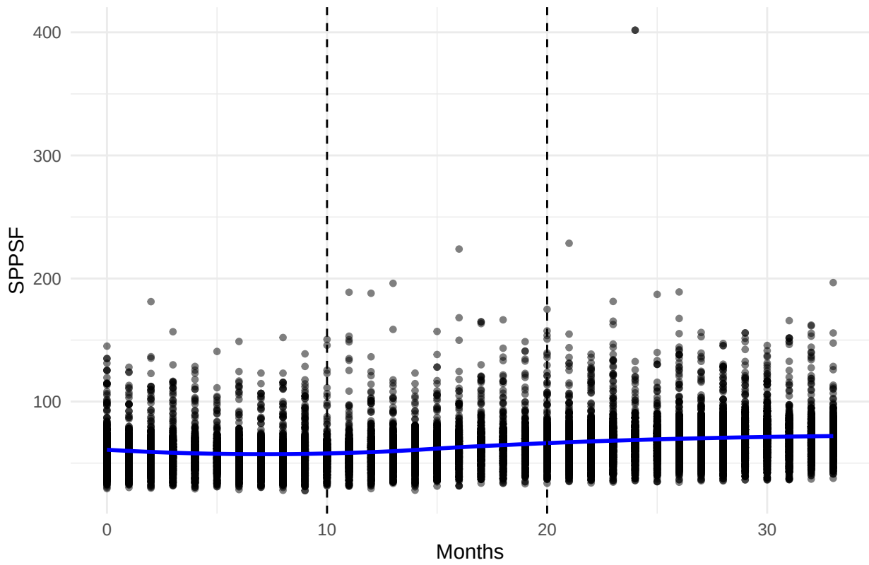
Months vs Predicted SPPSF – LN_SPPSF Model + Geo
