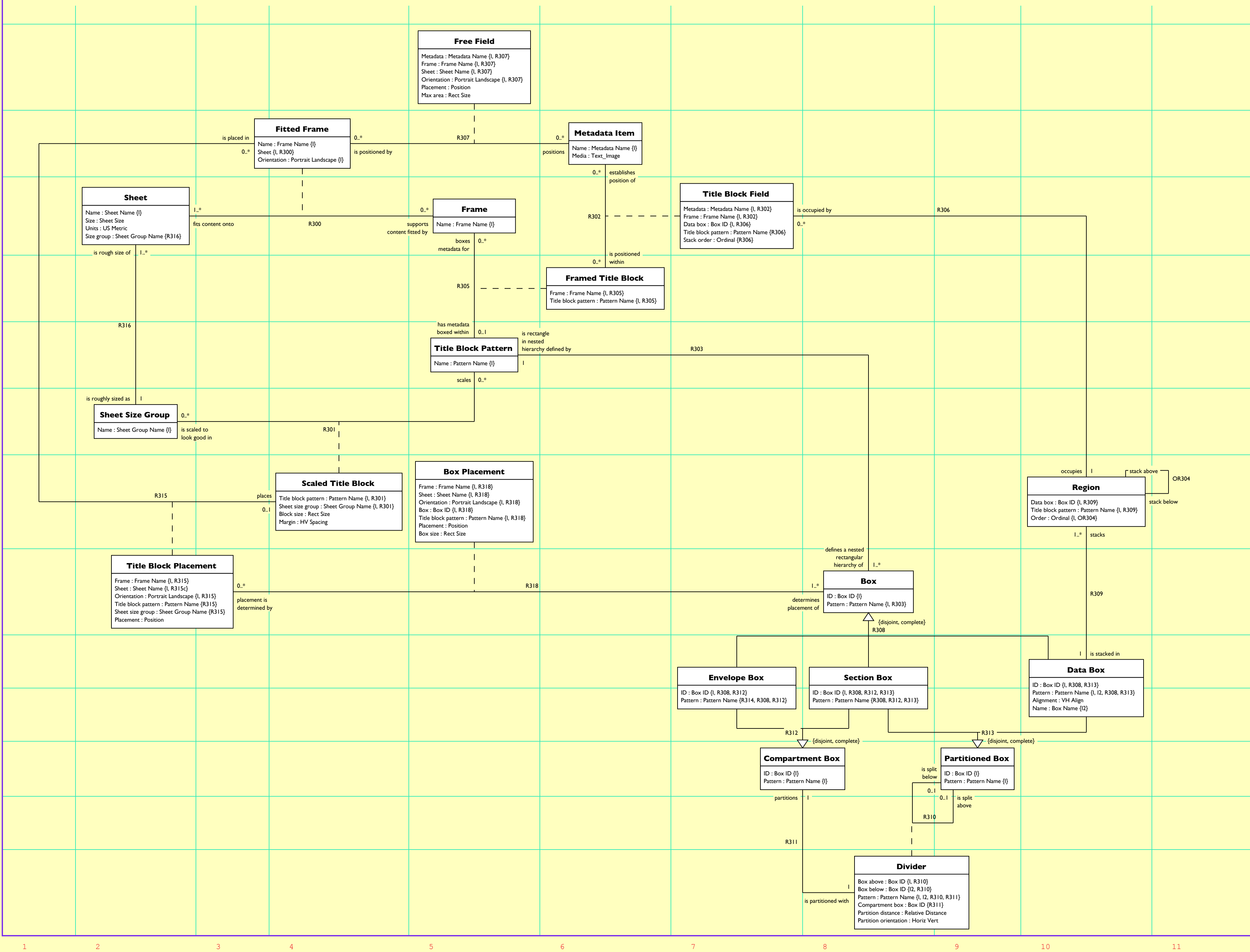
Flatland Sheet Subsystem Class Diagram
