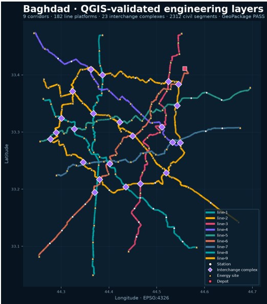
City-specific QGIS/GDAL package: 9 corridors, 182 stations, 23 interchanges and 2,312 classified civil segments.
