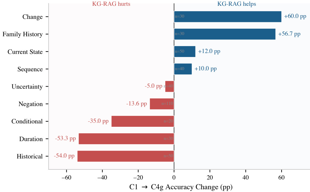
Figure 4: C1→C4g per-category accuracy change. Intent-aware KG-RAG produces large gains on categories requiring cross-admission normalization (change, family history) and losses on categories where the LLM’s parametric knowledge already suffices (historical, duration, conditional). Sample sizes per category shown.
