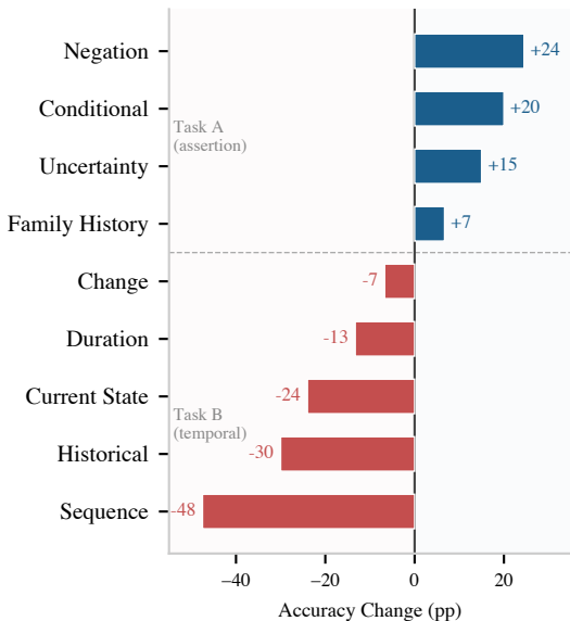
C3 -> C4 (+ assertions, no routing)
