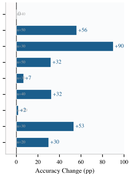
C1 to C4g (LLM alone to KG-RAG)
