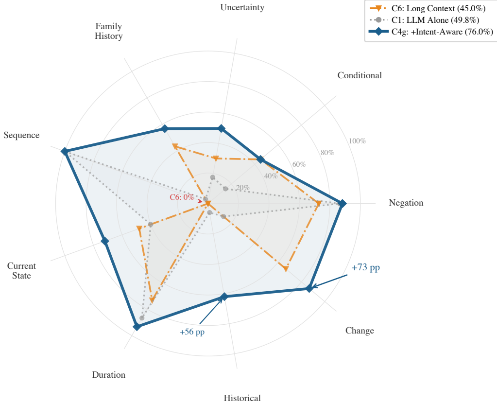
Figure 2: ClinicalBench per-category accuracy across three conditions (C6, C1, C4g; Claude Opus 4.6). C6 (orange dash-dot) collapses on historical and sequence (both 0%); C4g (dark solid) improves 8 of 9 categories over C1 with no regressions—the category×condition interaction that aggregate accuracy obscures.
