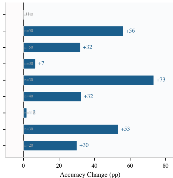
C1 to C4g (LLM alone to KG-RAG)
