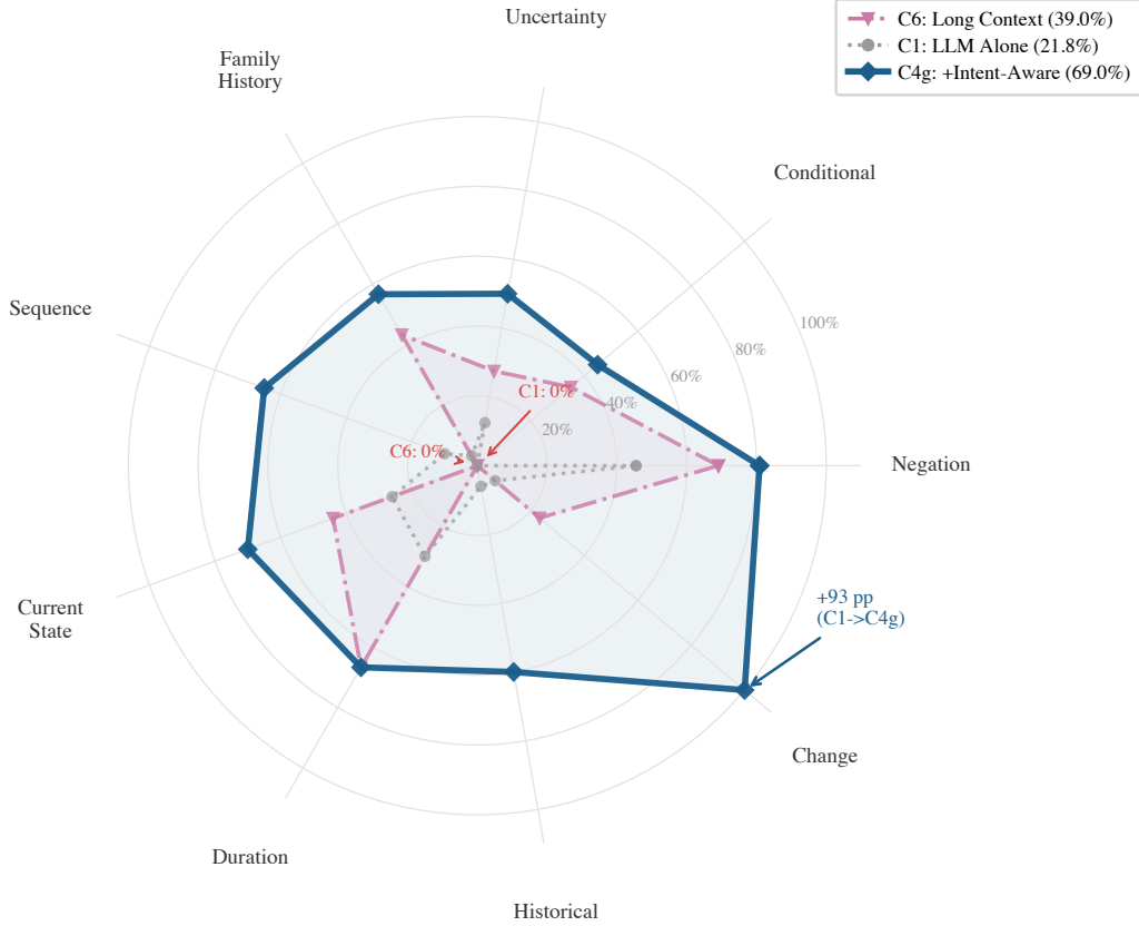
Figure 2: ClinicalBench per-category accuracy across three conditions (C6, C1, C4g; Claude Opus 4.6, evaluator v2). C6 (pink dash-dot) collapses on historical and sequence (both 0%); C1 (gray dotted) falls below 50% on 7 of 9 categories, reflecting frequent abstentions without retrieval context; C4g (dark solid) improves all 9 categories over C1.
