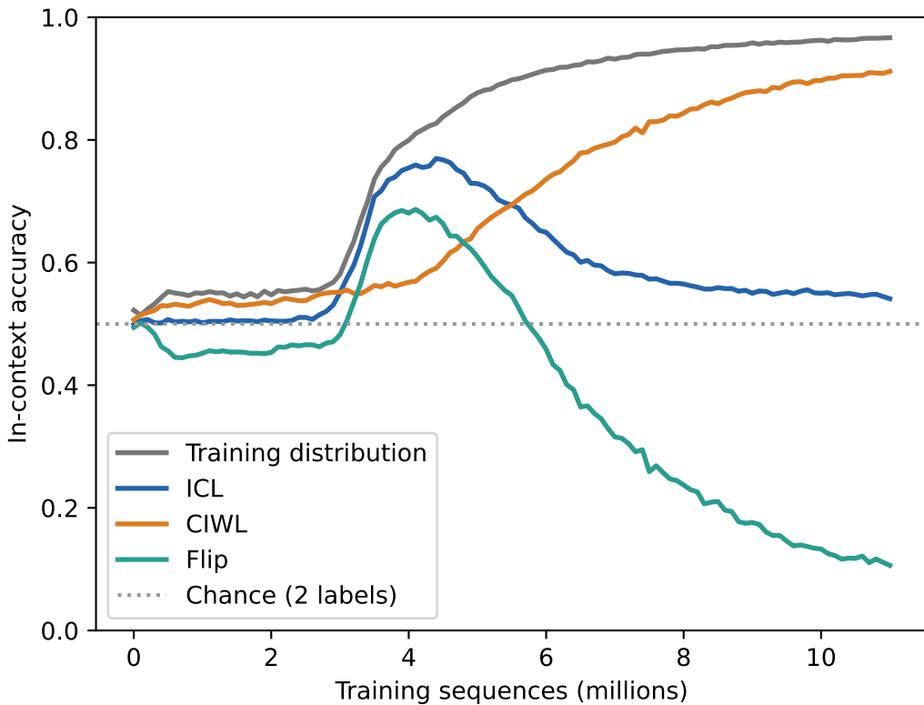
Main baseline in progress: through 11M sequences init seed 5 / train seed 2 / eval seed 1
