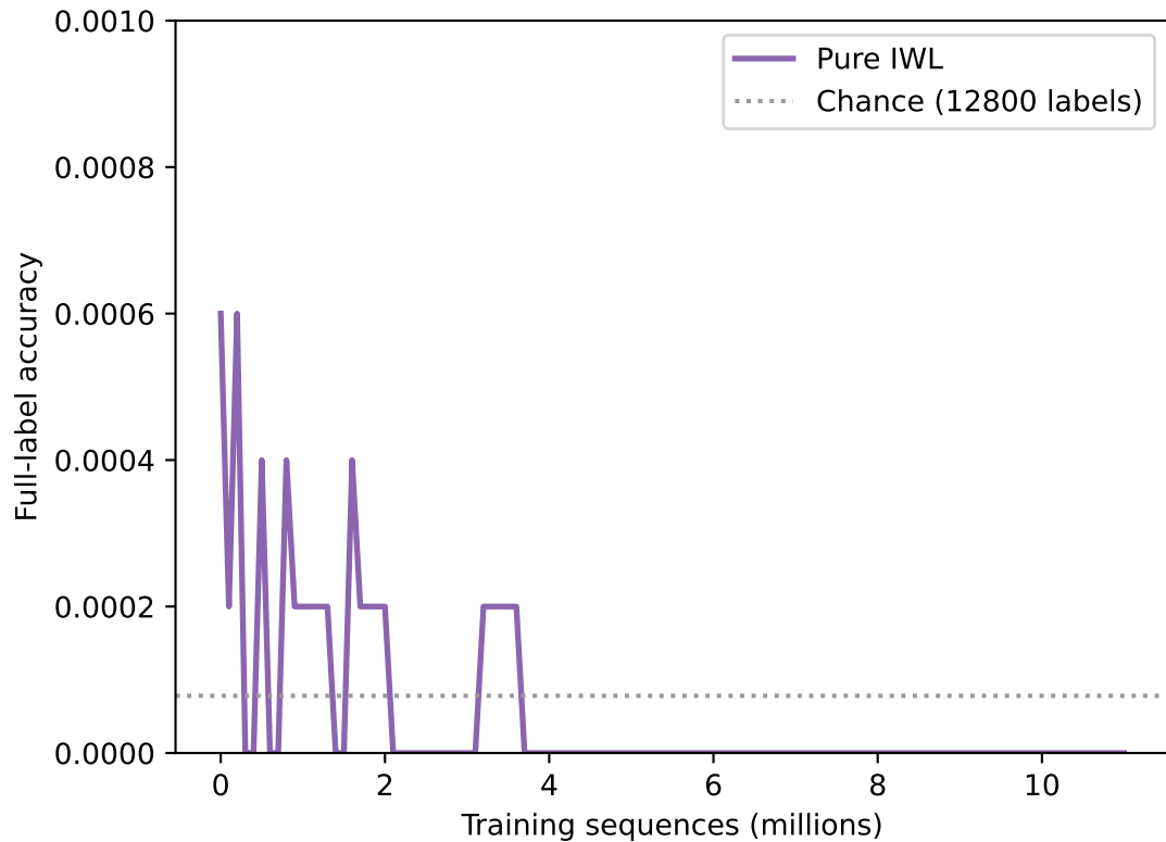
Main baseline in progress: through 11M sequences init seed 5 / train seed 2 / eval seed 1
