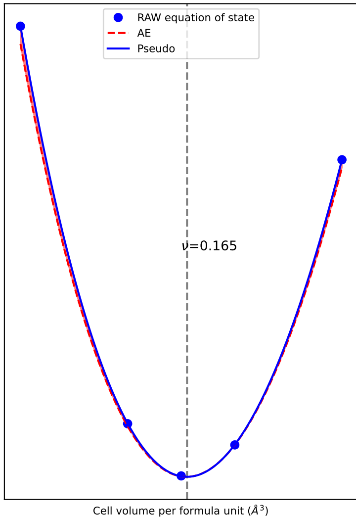
EOS of Diamond
