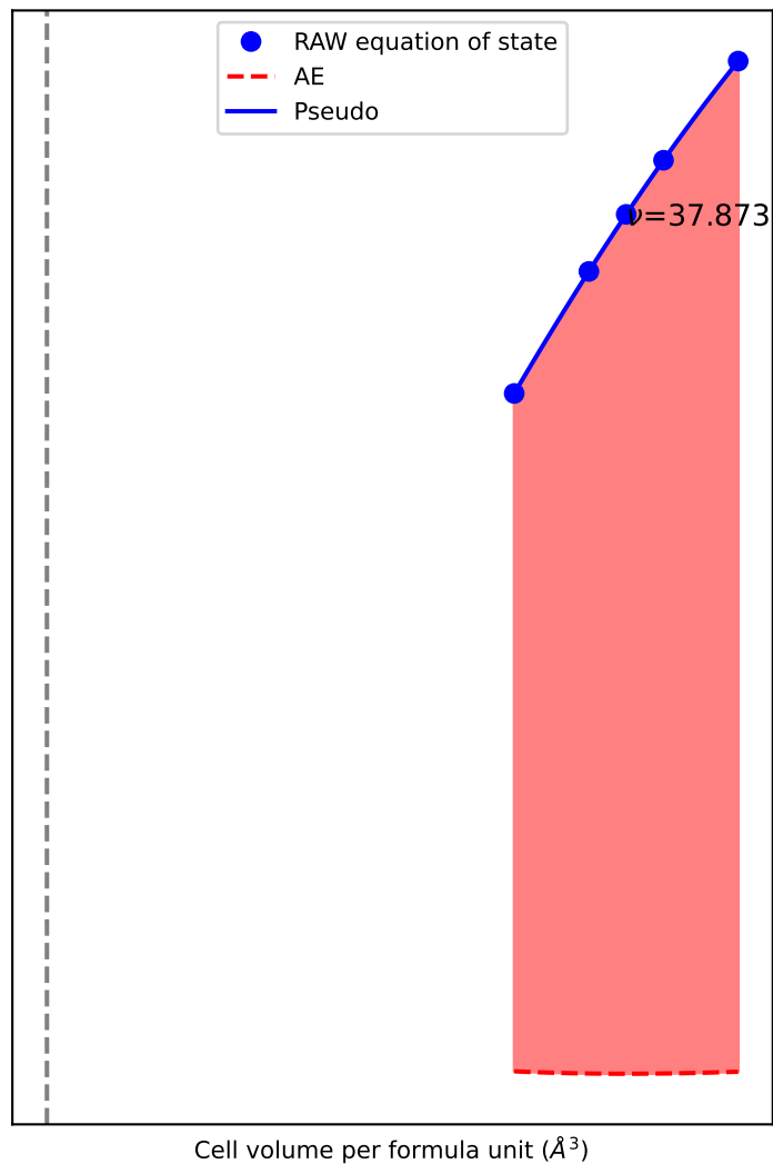
EOS of Diamond
