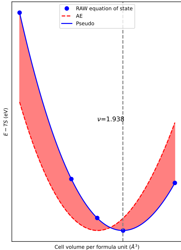
EOS of Diamond
