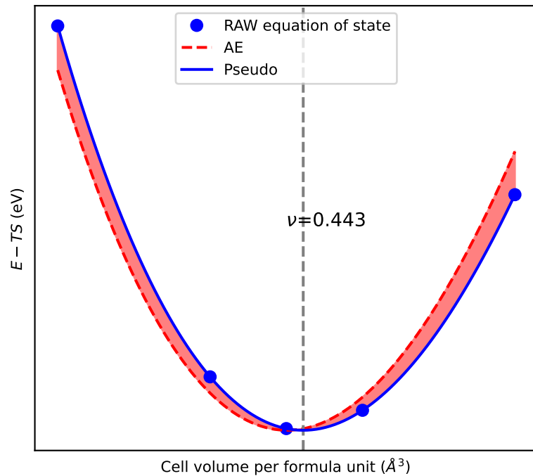
EOS of X2O5
