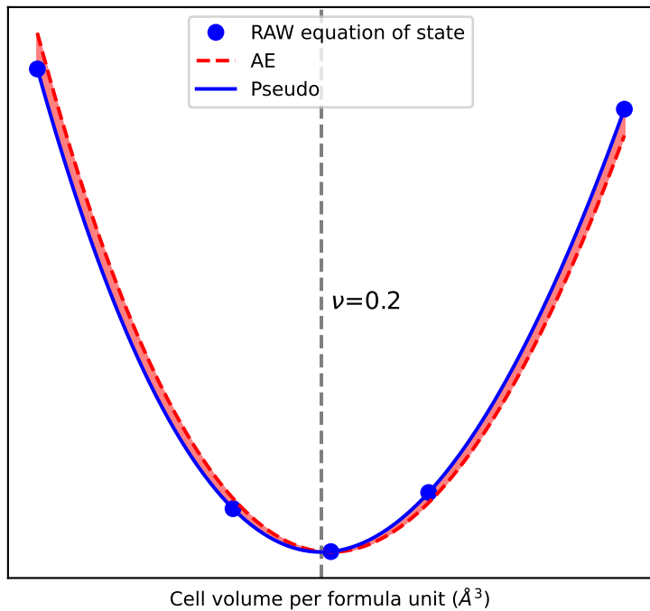
EOS of X2O3
