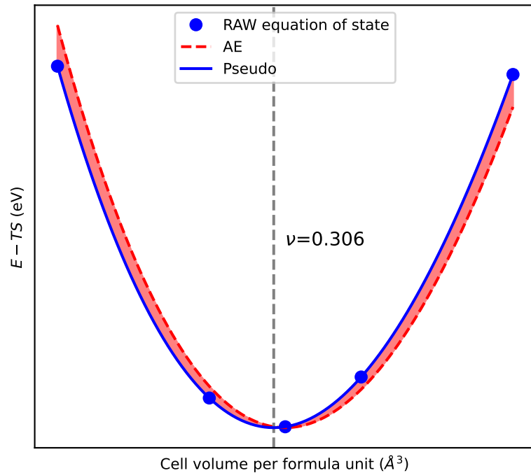
EOS of X2O
