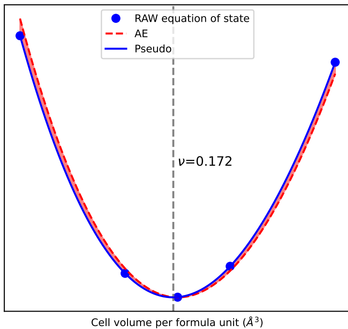
EOS of X2O3
