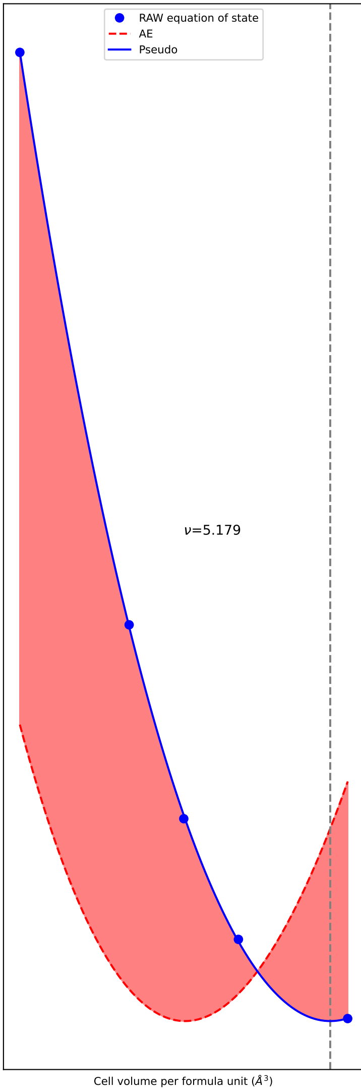
EOS of BCC
