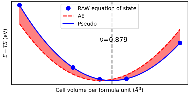
EOS of X2O3
