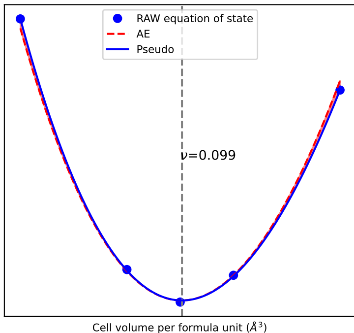
EOS of X2O
