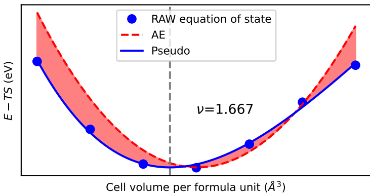
EOS of SC
