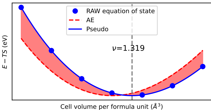
EOS of X2O3
