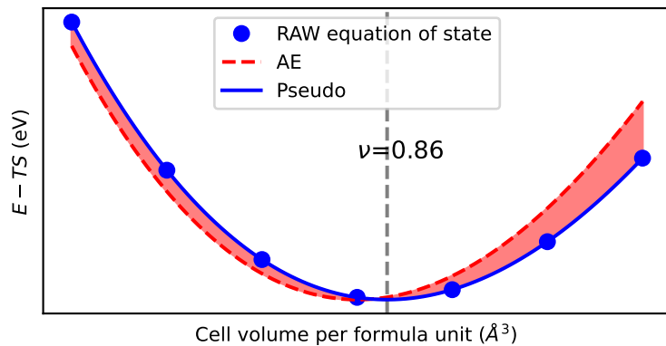
EOS of X2O
