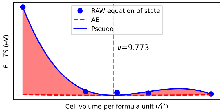
EOS of X2O5
