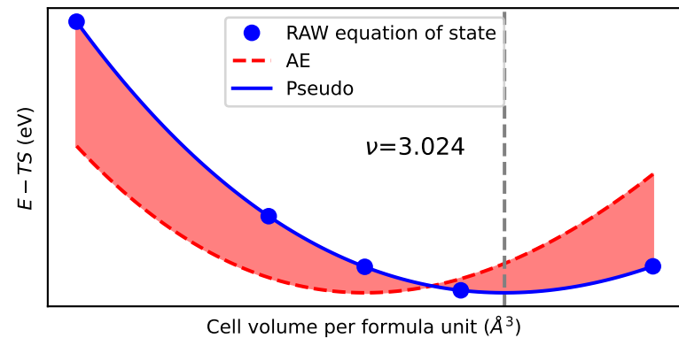
EOS of X2O3
