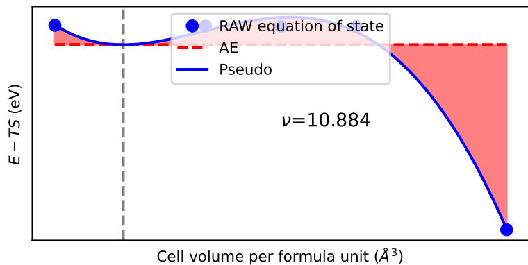
EOS of Diamond
