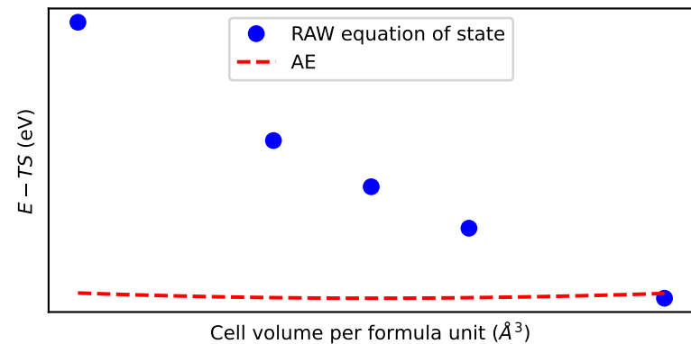
EOS of SC
