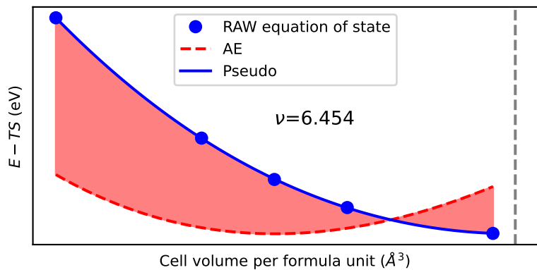
EOS of X2O
