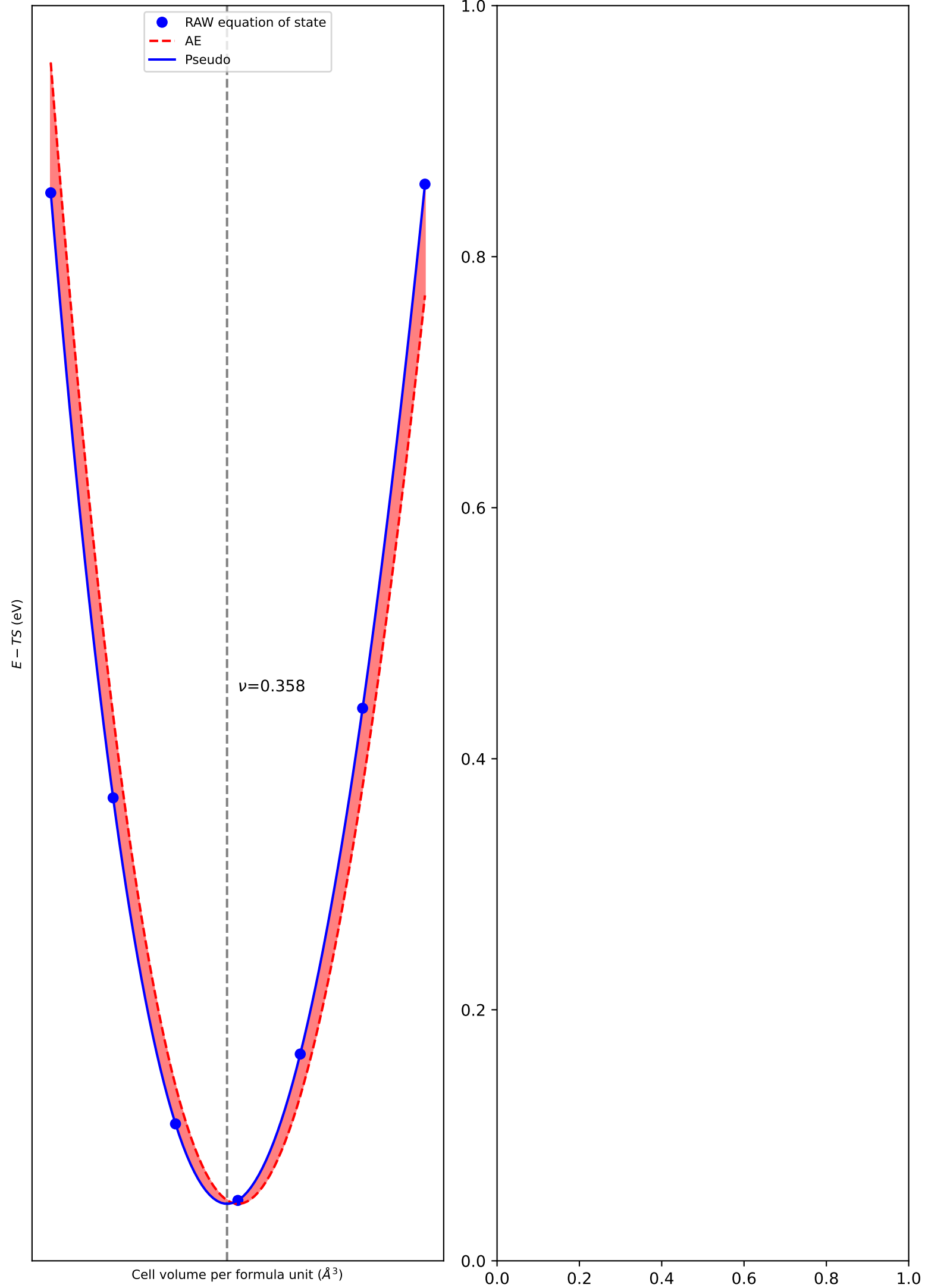
EOS of X2O5
