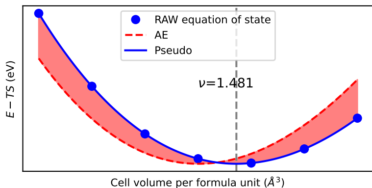
EOS of FCC
