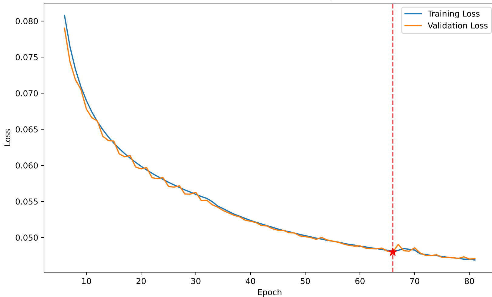
Loss 0.048 vs Val Loss 0.048 at epoch 66
