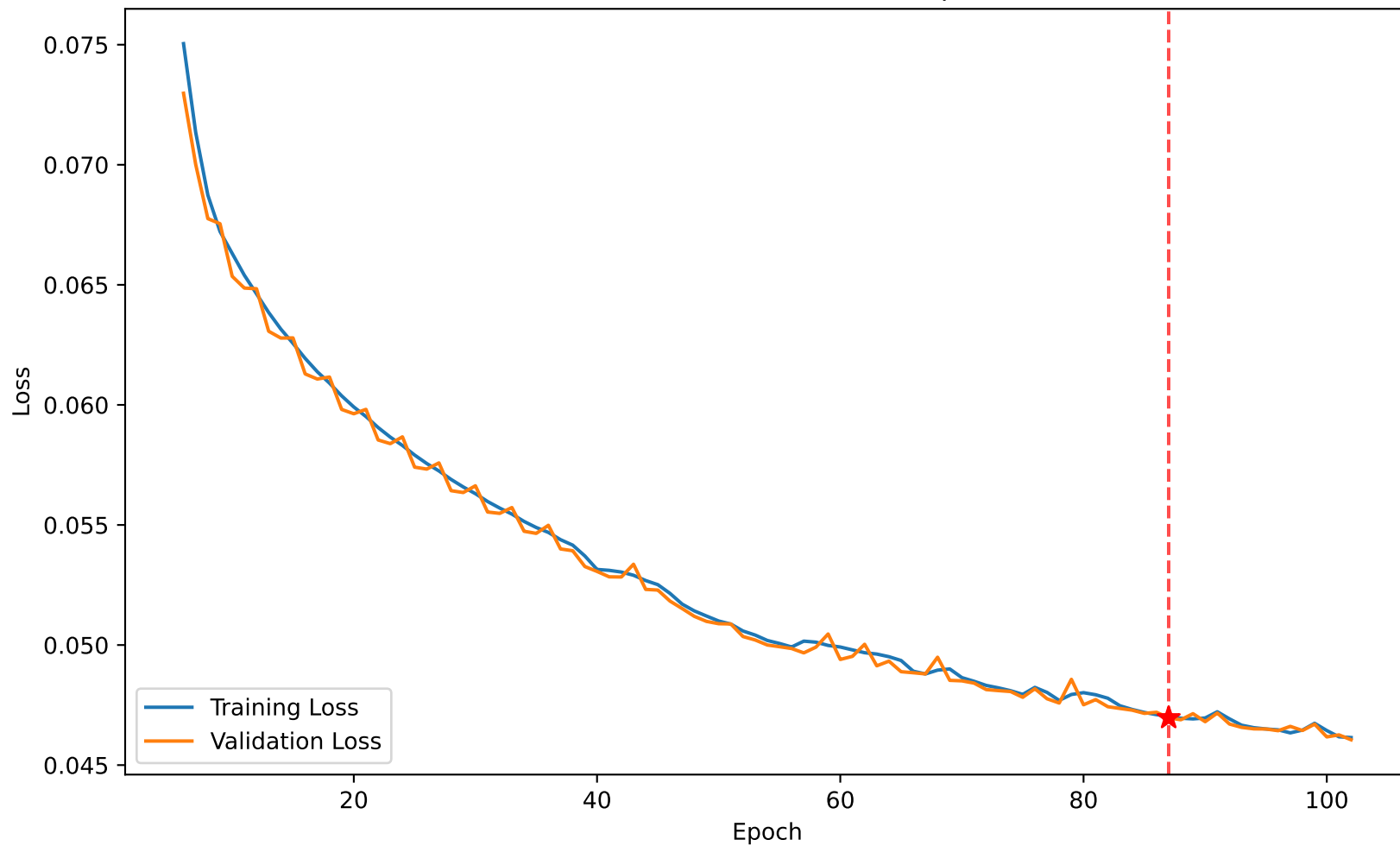
Loss 0.047 vs Val Loss 0.047 at epoch 87
