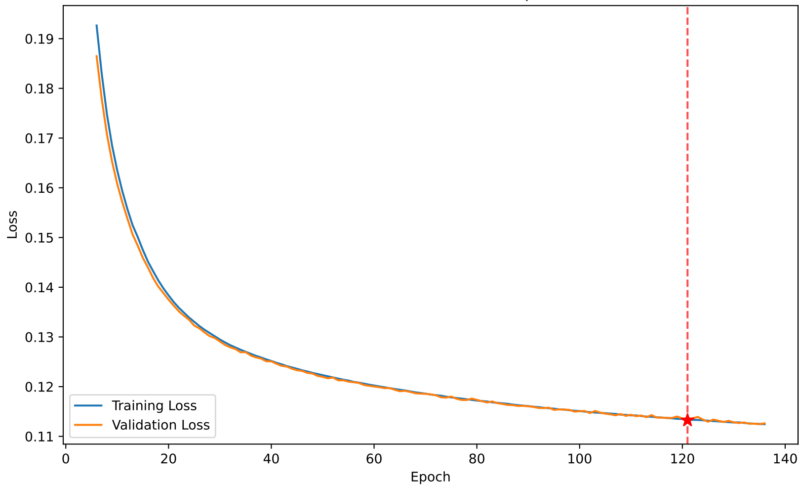
Loss 0.113 vs Val Loss 0.113 at epoch 121
