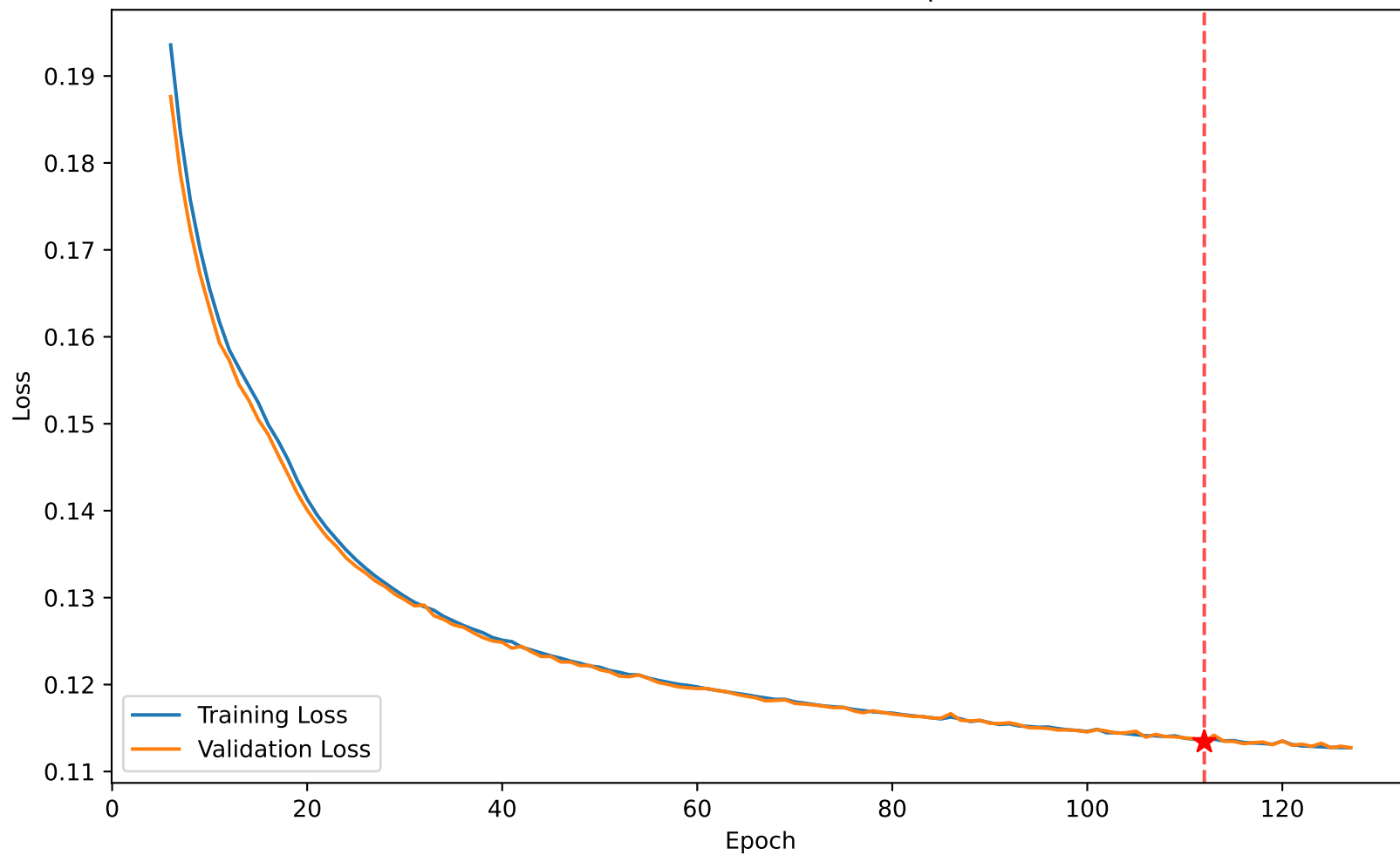
Loss 0.114 vs Val Loss 0.113 at epoch 112
