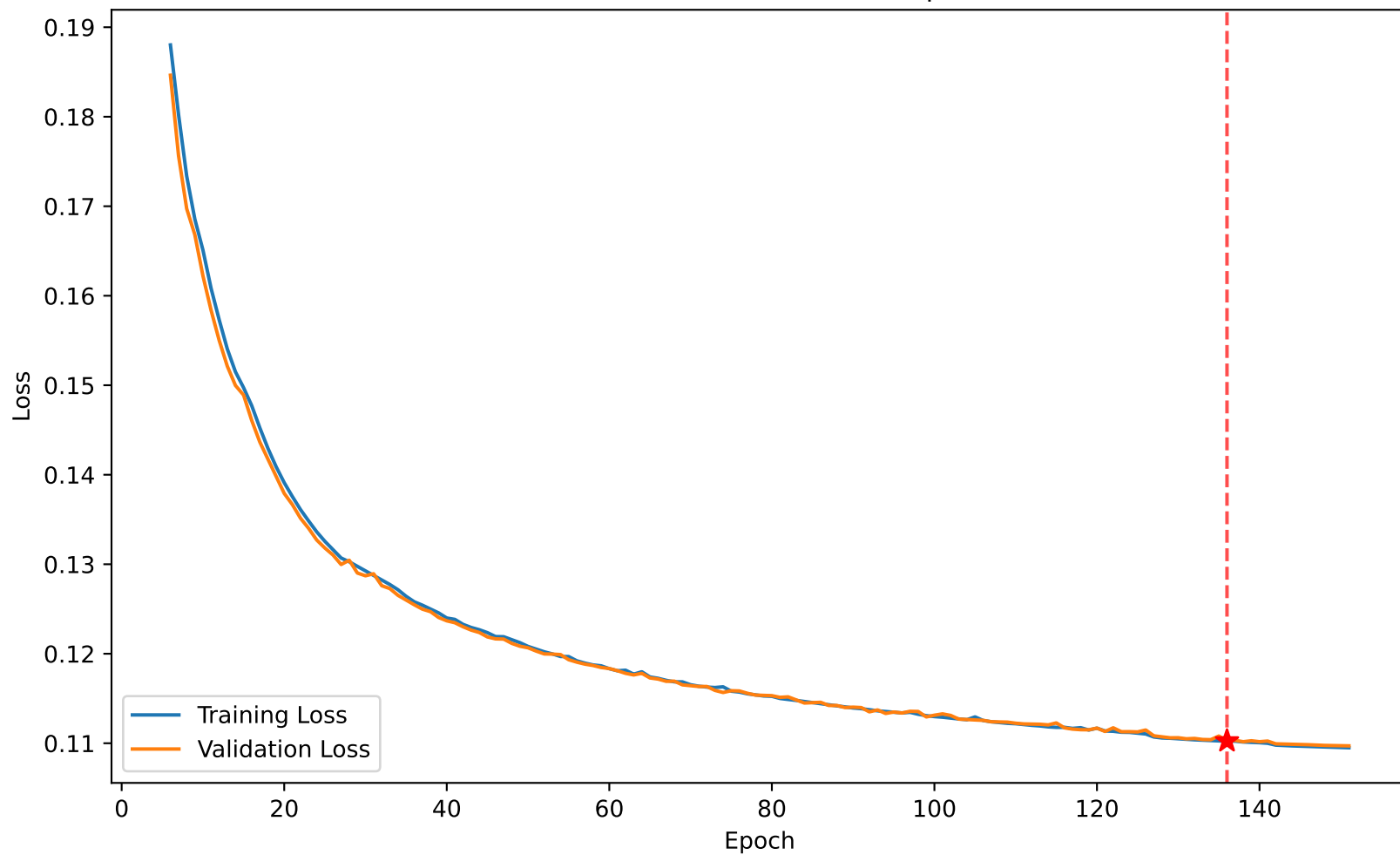
Loss 0.110 vs Val Loss 0.110 at epoch 136
