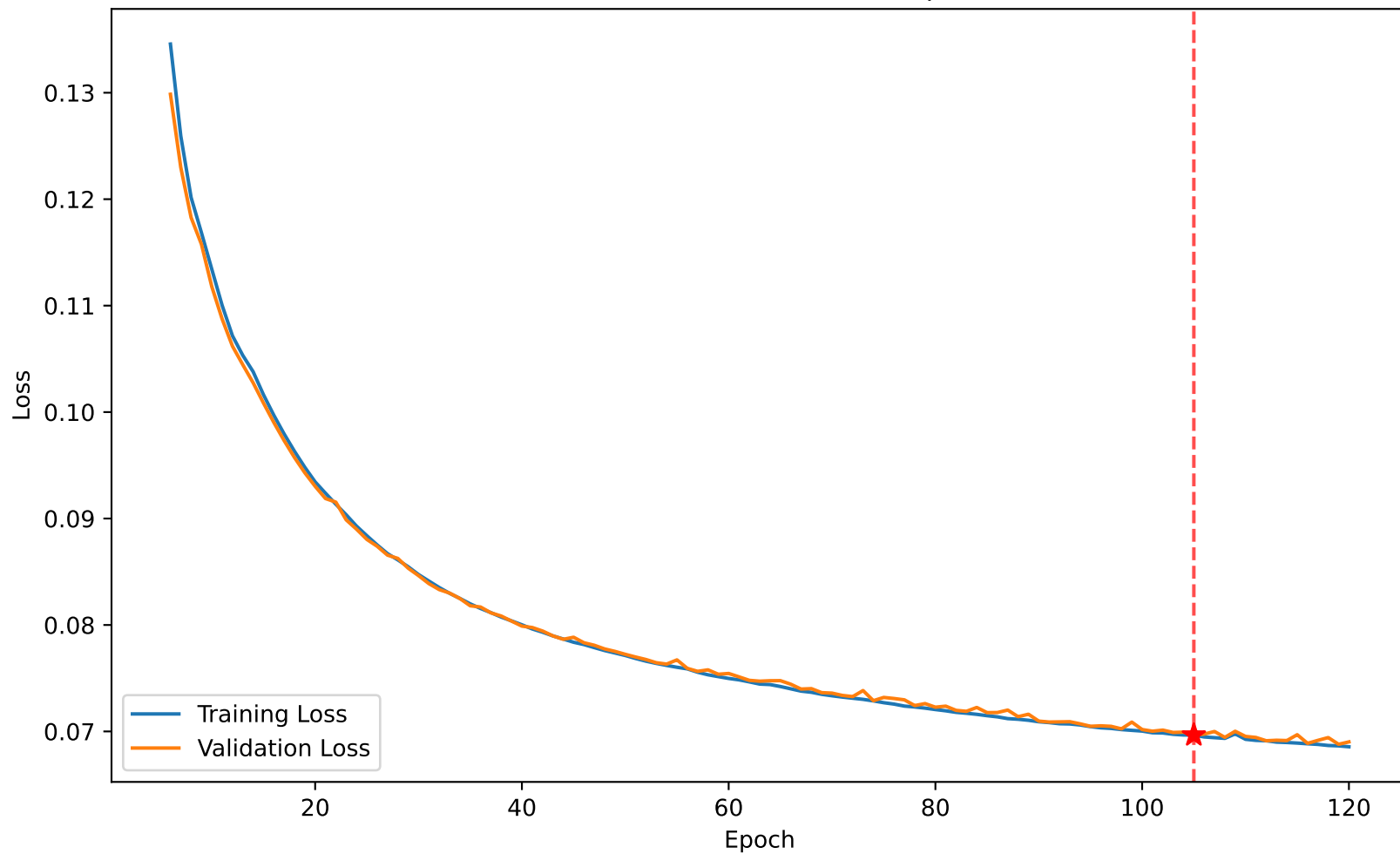
Loss 0.070 vs Val Loss 0.070 at epoch 105
