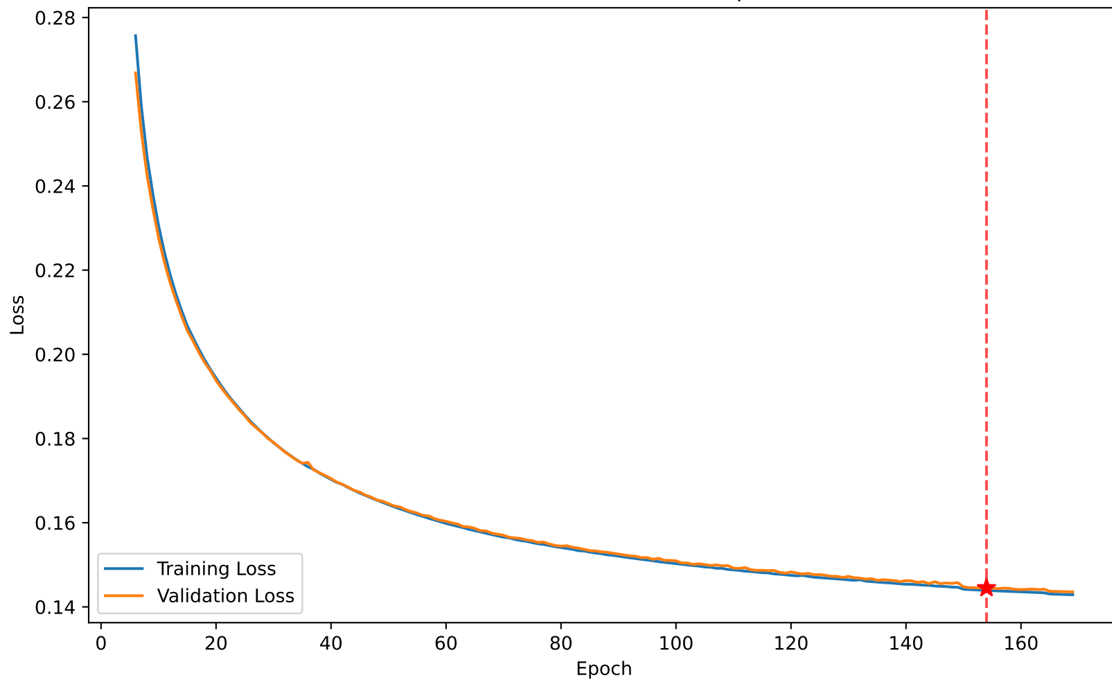
Loss 0.144 vs Val Loss 0.145 at epoch 154
