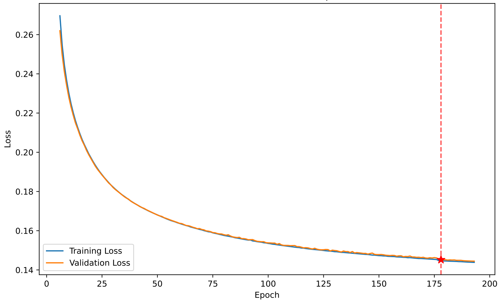
Loss 0.145 vs Val Loss 0.145 at epoch 178
