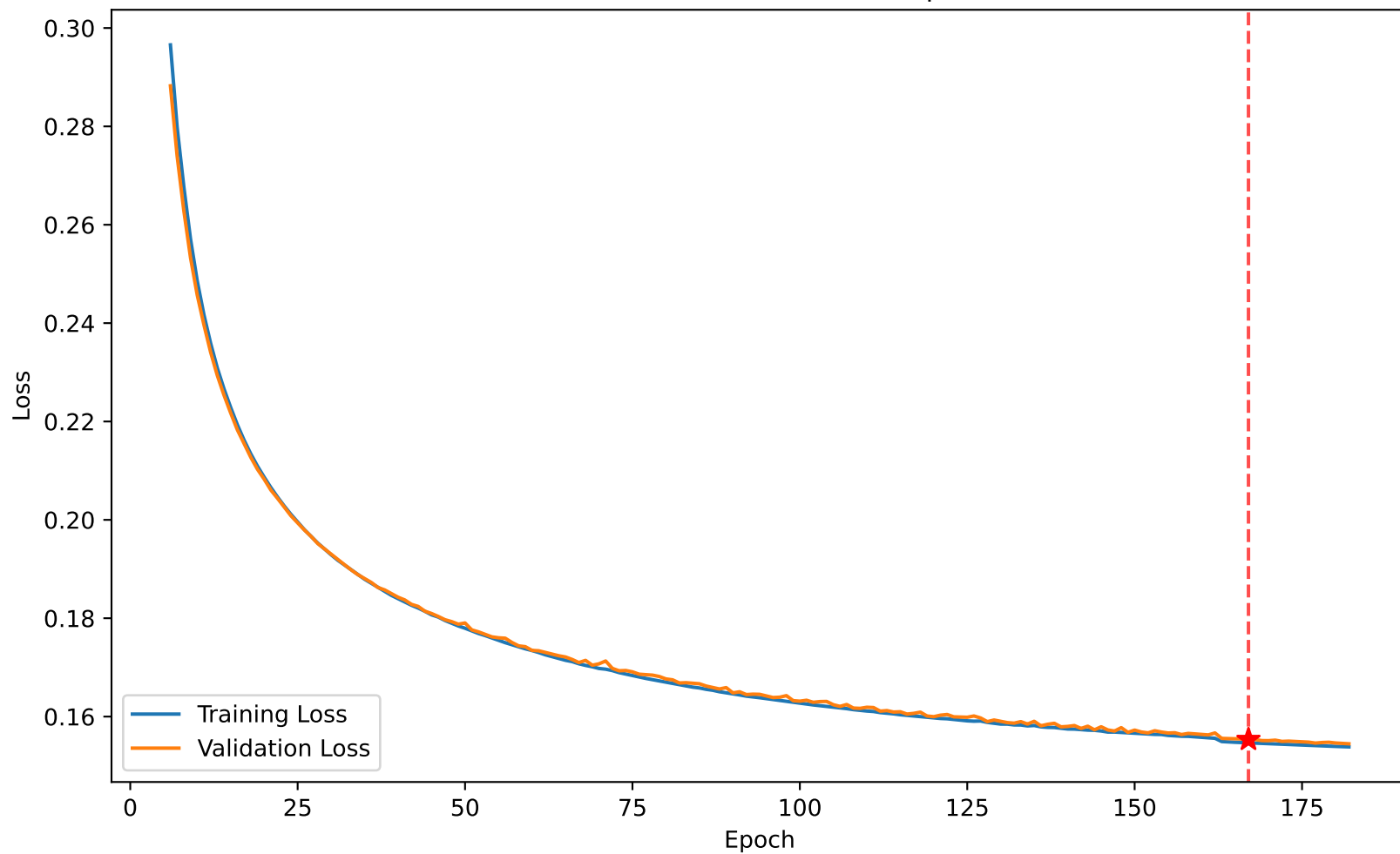
Loss 0.155 vs Val Loss 0.155 at epoch 167
