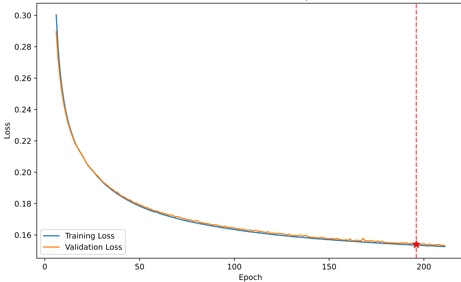
Loss 0.154 vs Val Loss 0.154 at epoch 196
