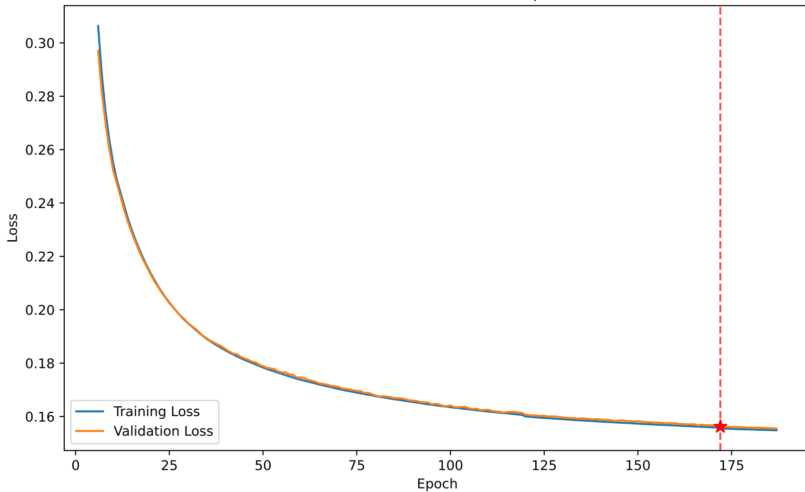
Loss 0.156 vs Val Loss 0.156 at epoch 172
