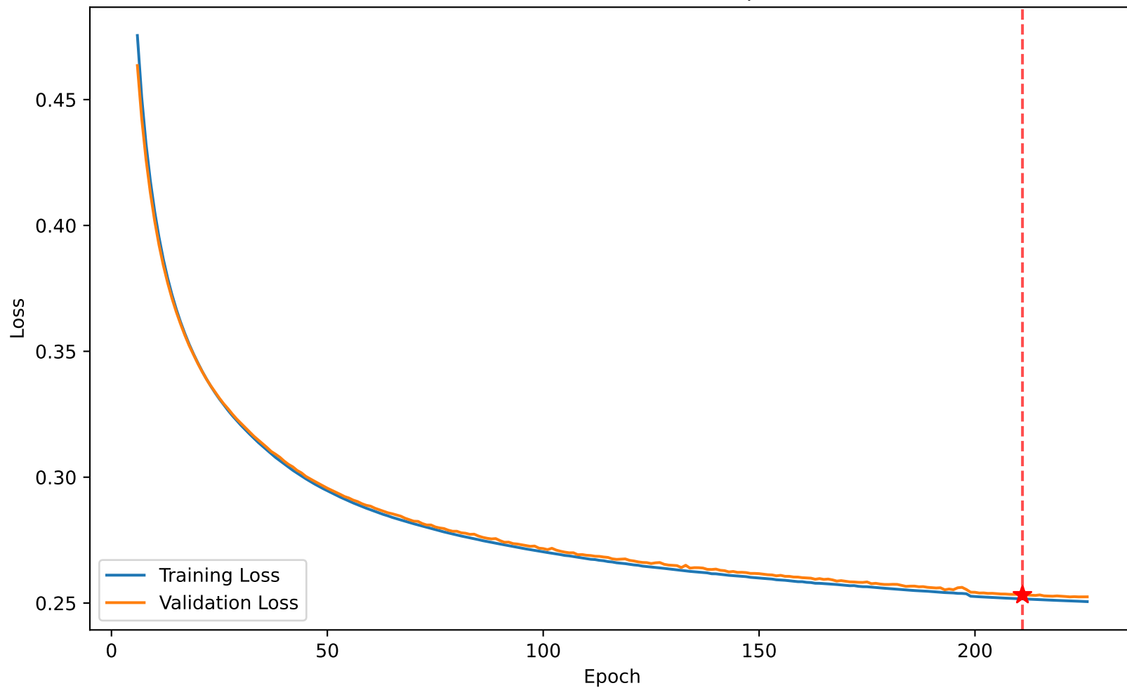
Loss 0.252 vs Val Loss 0.253 at epoch 211
