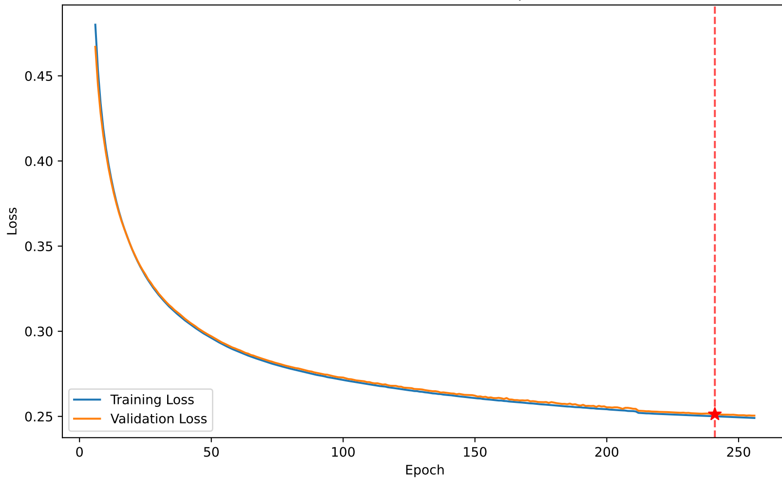
Loss 0.250 vs Val Loss 0.251 at epoch 241
